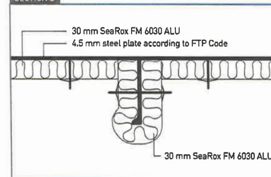
SECTION D
