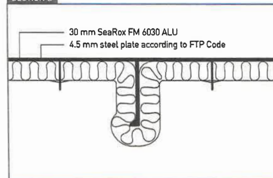
SECTION B
