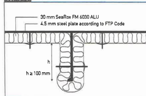
SECTION C
